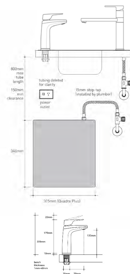
XL Levered tap dimensions
